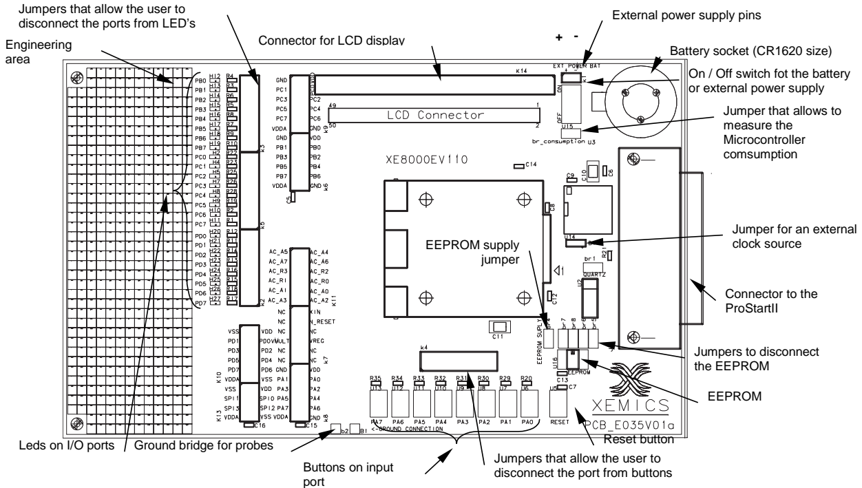
Figure 2 Board elements
